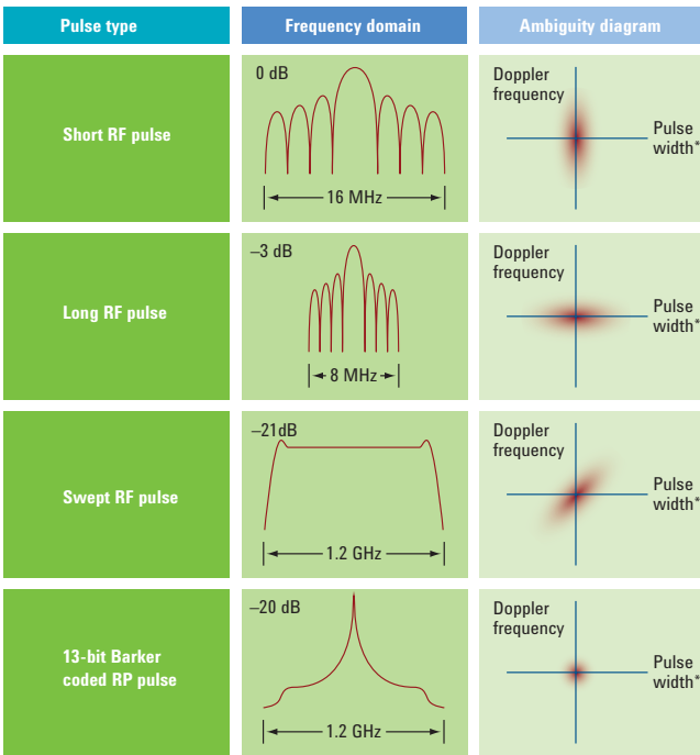
Figure 1. An ambiguity diagram illustrates location accuracy versus Doppler accuracy. This figure shows relative ambiguity diagrams for different types of radar pulses.
