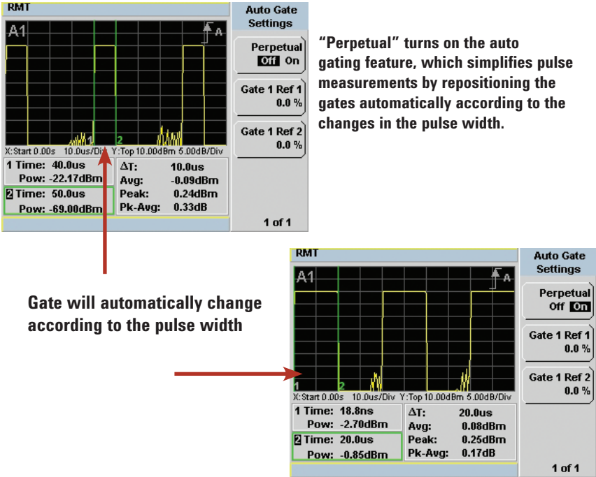
Figure 9. The P-Series power meter has the capability to directly measure pulse power by automatically positioning a gate on a pulse.
